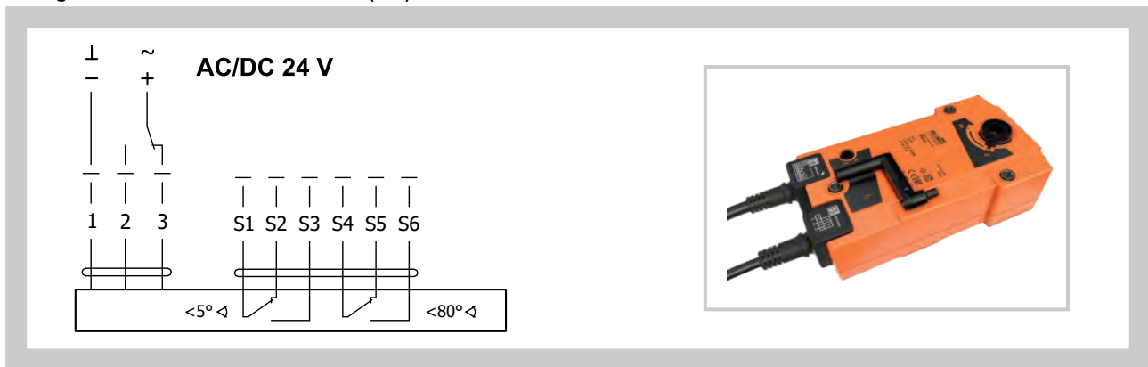
Fig. 10 Actuator BELIMO BEE 24(-ST)
